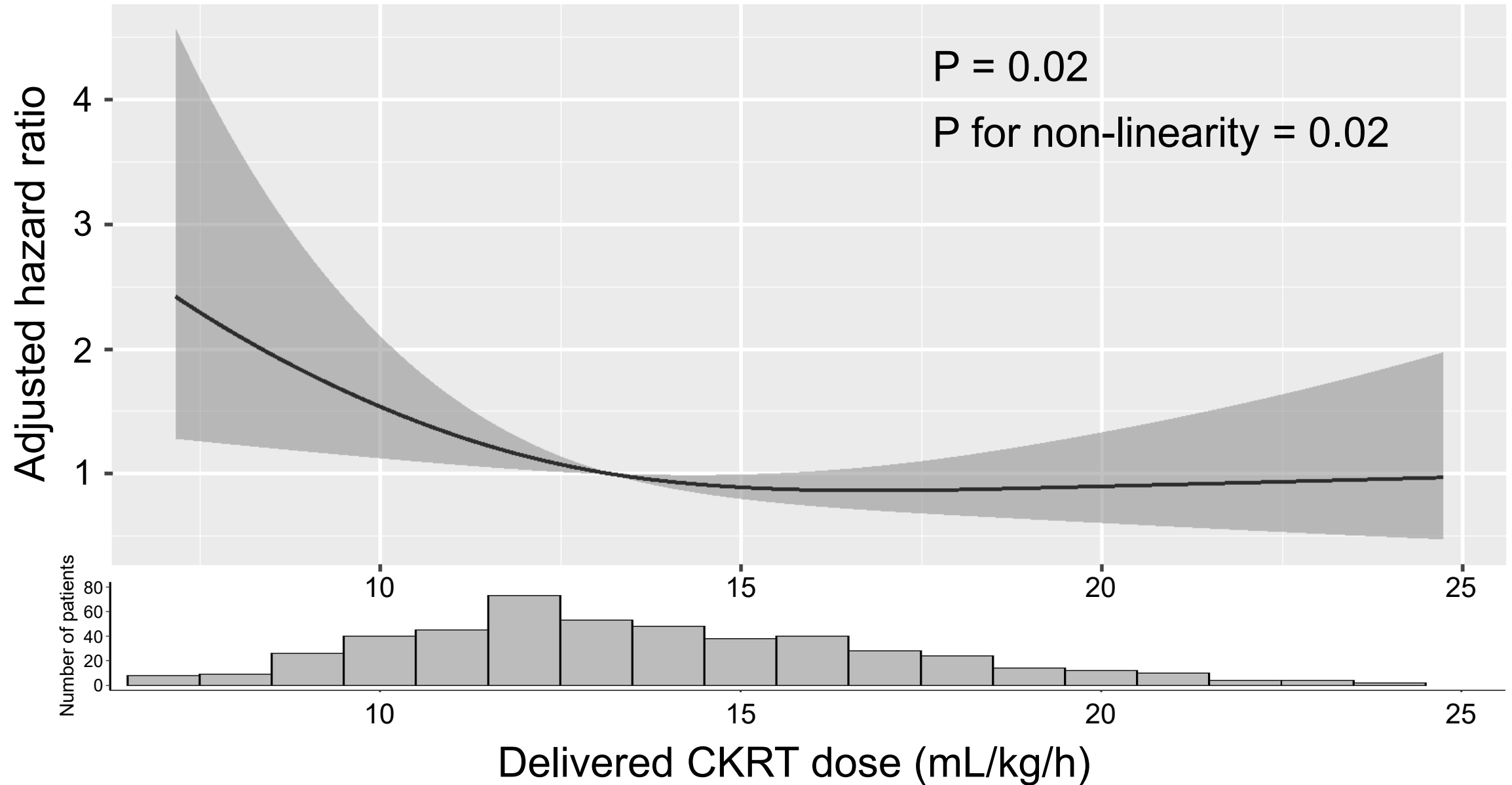
Figure 3. Association between adjusted HR for 90-day mortality and delivered CKRT dose: restricted cubic spline with 3 knots.
